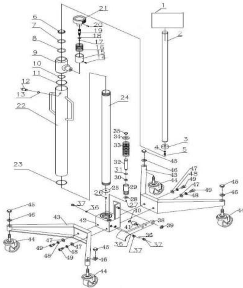
Parts List AND DIAGRAM(UPPER UNIT)
